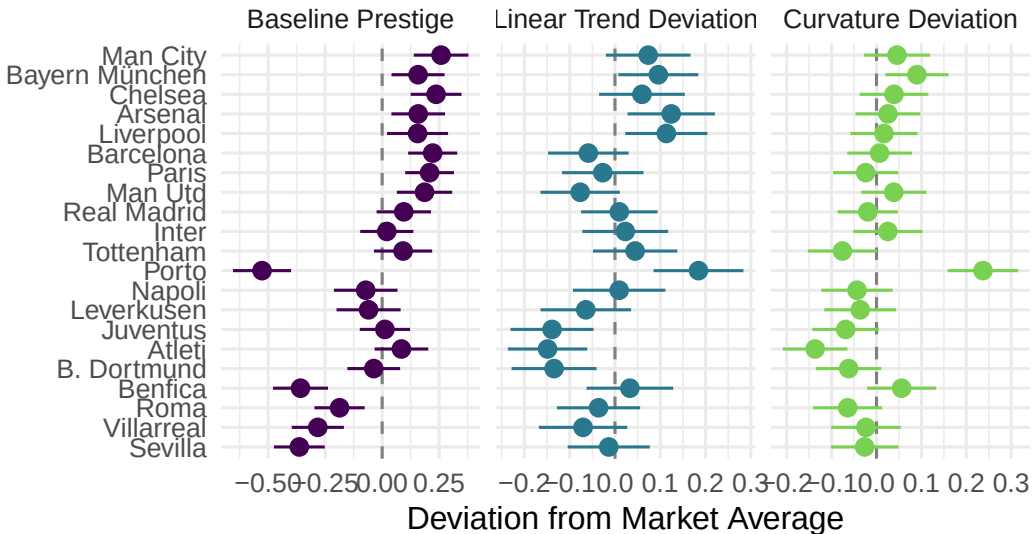
Figure 6. Club-Level Trajectory Deviations Estimates from Model 3.2 (Orthogonal Polynomials)
